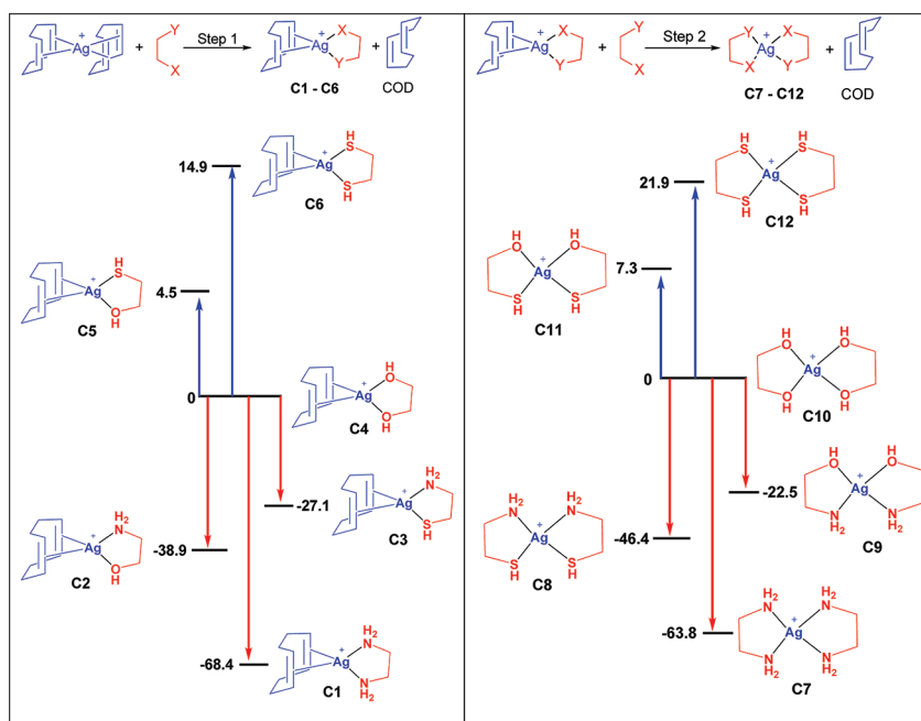
FIGURE 2. Relative complex formation energy for the stepwise displacement of COD by dinucleophile. Diagram drawn with reference to the formation energy of (i) C4 ( -67.8 \text{ kJ mol}^{-1} ) as zero in step 1 (left) and (ii) C10 ( -8.8 \text{ kJ mol}^{-1} ) as zero in step 2 (right). Details in the Supporting Information.
