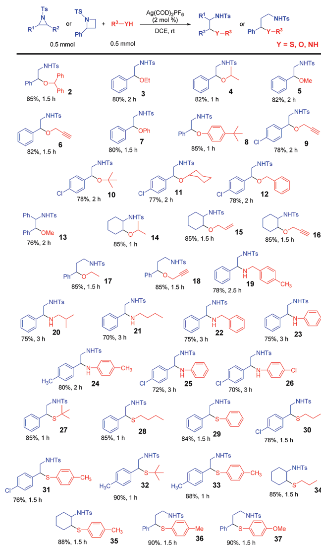
FIGURE 3. Substrate scope for Ag(I)-catalyzed regioselective ring-opening of N -tosylaziridine and N -tosylazetidine with N -, O -, and S -nucleophiles. Yield refers to isolated yields of pure products.
